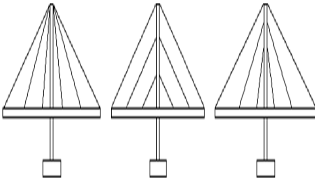
Fig 2 Cable Arrangements a) Radial b) Harp c) Fan
