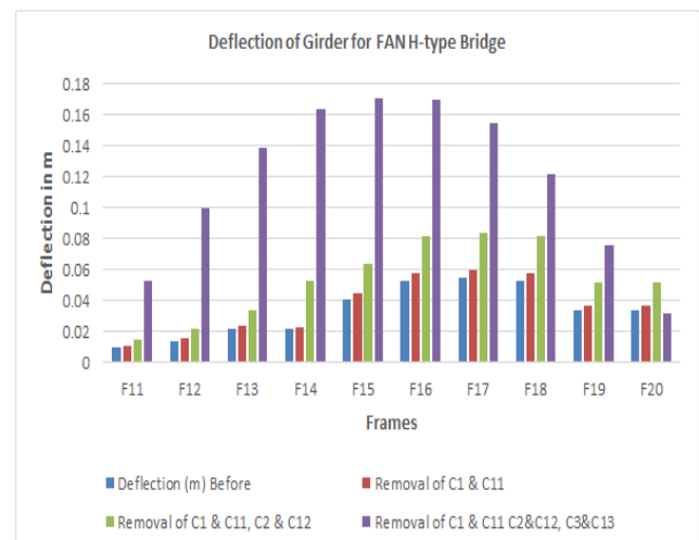
Fig 6. Deflection of Girder for FAN H-type Bridge
