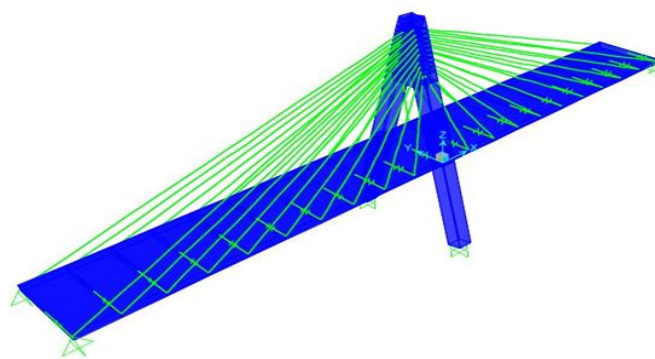
Fig 4. Fan Cable arrangement with A-type pylon
