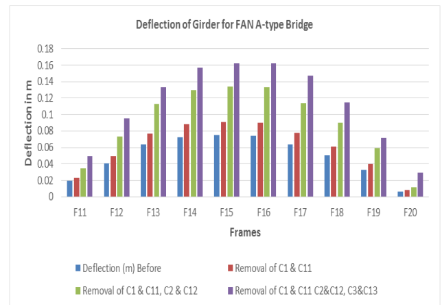
Fig 5. Deflection of Girder for FAN A-Type Bridge
