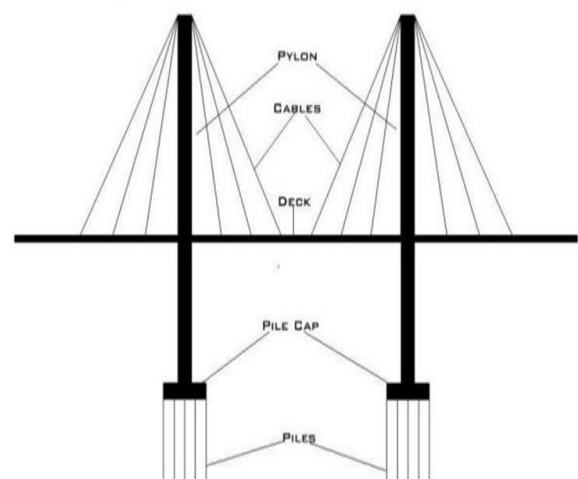
Fig 1. Components of Cable Stayed Bridge
