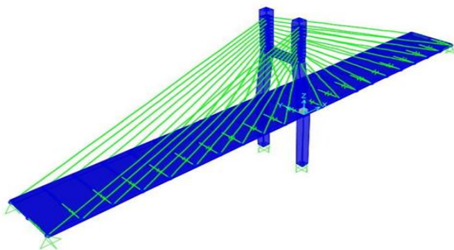
Fig 3. Fan Cable arrangement with H-type pylon
