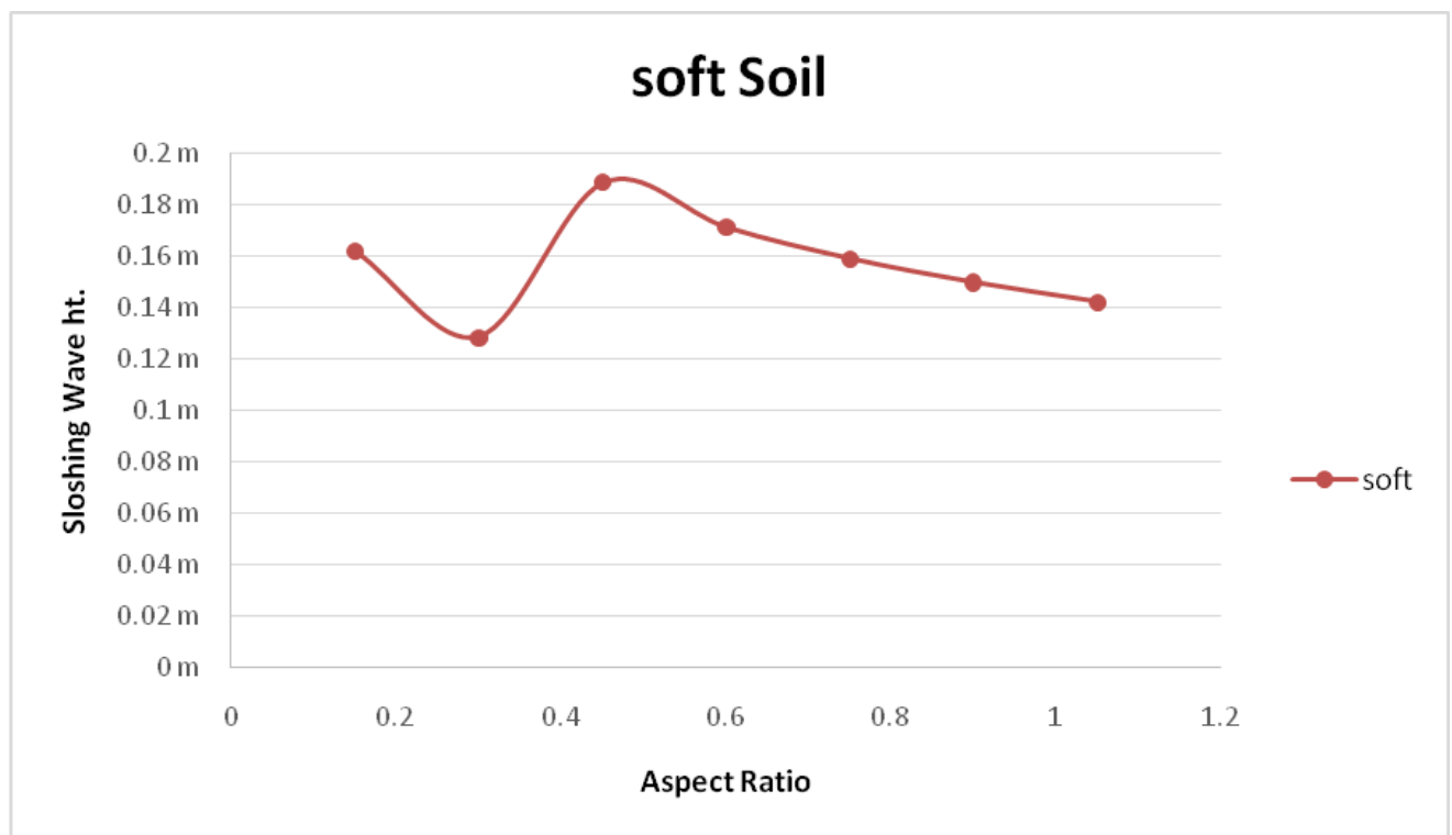
Graph 2: Sloshing wave height behaviour in Soft Soil
