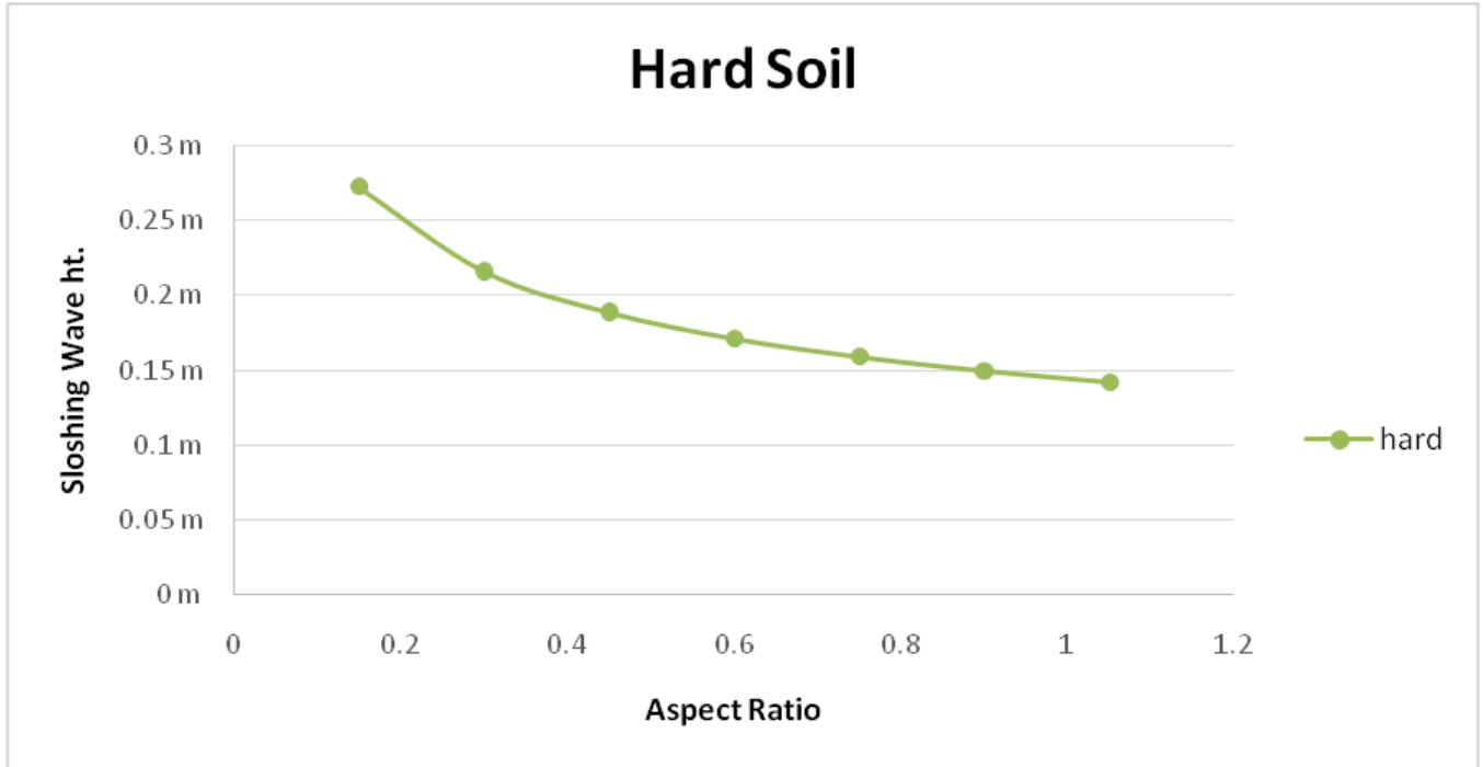
Graph 3- Sloshing wave height behaviour in Hard Soil.
