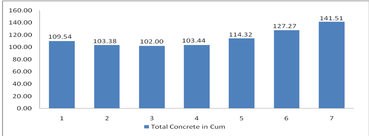
Graph 6 - Quantity of Concrete in all Seven Tanks.
