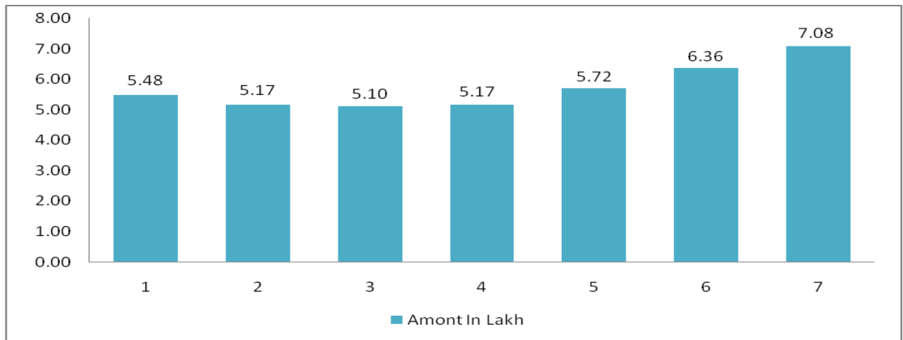
Graph 7 - Cost of Concrete in all Seven Tanks.
