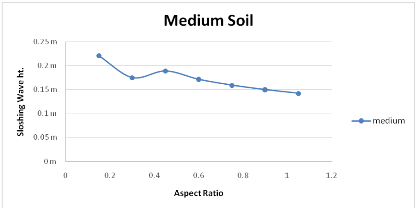
Graph 4 Sloshing wave height behaviour in Medium Soil.
