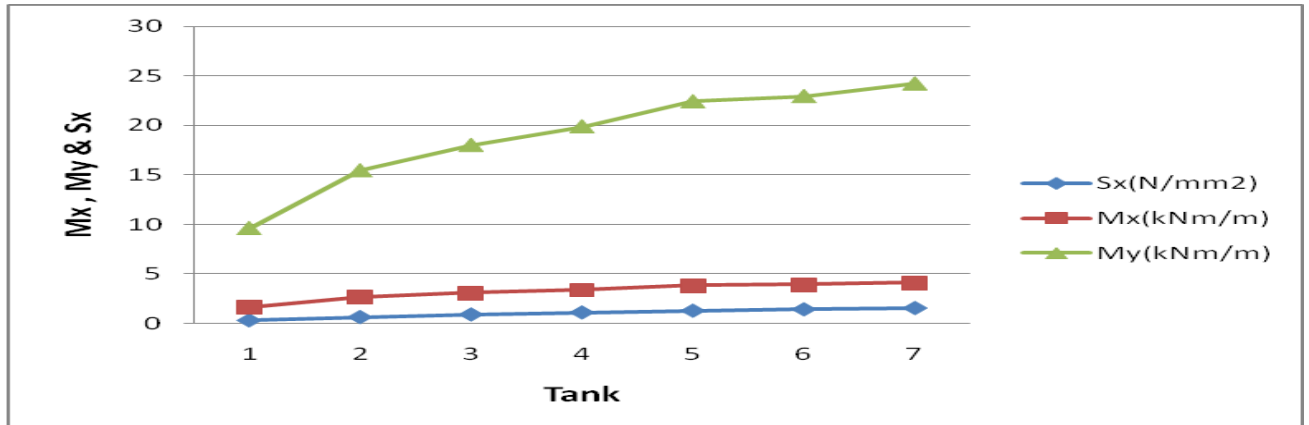
Graph 1 Moments & Shear forces behaviour in Hydro Test + Seismic.
